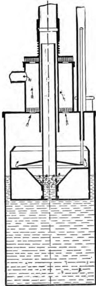
FIG. 151.—The Daimler Filtering Carburettor, used on the early Daimler cycles and carriages.
